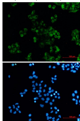
Immunocytochemistry analysis of DAB2 (green) in HeLa using DAB2 antibody, and DAPI (blue)
