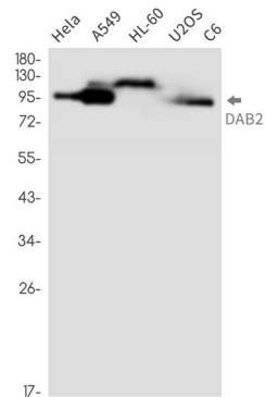
Western blot analysis of DAB2 in HeLa, A549, HL-60, U2OS, C6 lysates using DAB2 antibody.
