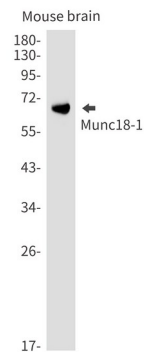
Western blot analysis of Munc181 in mouse brain lysates using Syntaxin Binding Protein 1 antibody.
