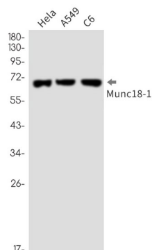
Western blot analysis of Munc181 in HeLa, A549, C6 lysates using Munc181 antibody.
