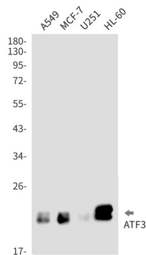
Western blot analysis of ATF3 in A549, MCF-7, U251, HL-60 lysates using ATF3 antibody.
