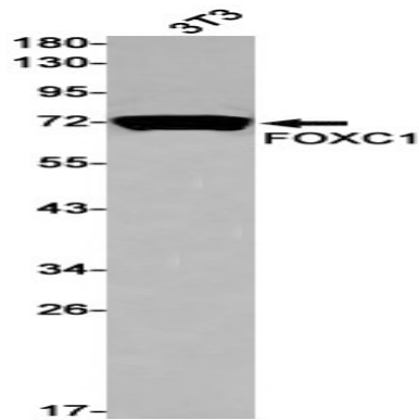
Western blot analysis of FOXC1 in 3T3 lysates using FOXC1 antibody.
